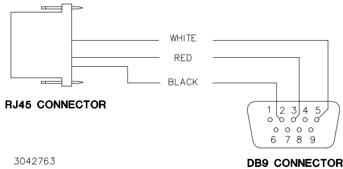
FIGURE 1. RJ45 TO DB9 ADAPTER WIRING
